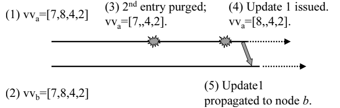
Figure 5: The second problematic case. Initially, in steps (1) and (2), the state of node a and b is identical. In step (3), because node a 's clock is faster than b 's, the second entry in vv_a is pruned before vv_b 's. Later, in step (4), node a issues a new update 1 that "happens-after" the update currently stored in both a and b . When update 1 arrives at node b , b detects a false conflict.
