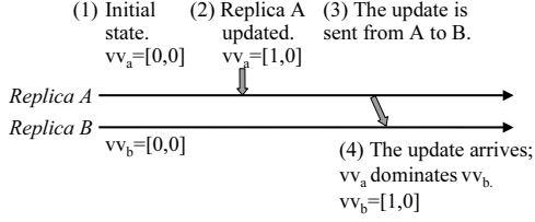
Figure 2: In this example, two replicas, a and b , start from the identical state in step (1), with version vectors [0,0] (i.e., entries for a and b both being 0). Replica a is updated in step (2), and the update is sent to b in step (3). Since a is strictly newer than b , replica b detects no conflict in step (4).
