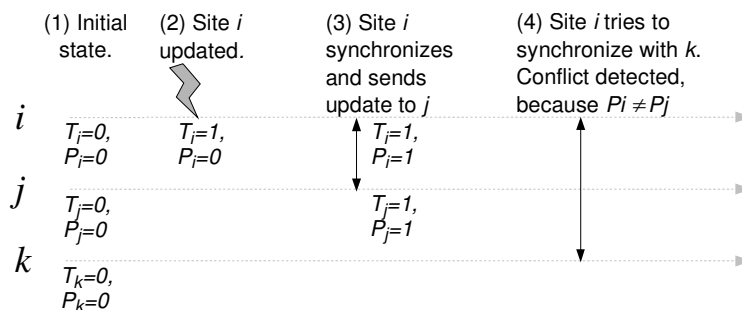
Fig. 12. An example of erroneous conflict detection using the two-timestamp algorithm. A lightning bolt shows the submission of an operation, and an arrow shows bidirectional operation propagation. T_x shows the current timestamp of replica x (noted ts in Figure 11), and P_x show its previous timestamp (i.e., prevTs ). Initially in (1), the contents of the replicas are identical, with T_x = P_x = 0 for all the replicas. In step (4), Replicas i and k try to synchronize. The algorithm incorrectly detects a conflict, because P_i (= 2) \neq P_k (= 0) . In reality, Replica k is strictly older than Replica i .
